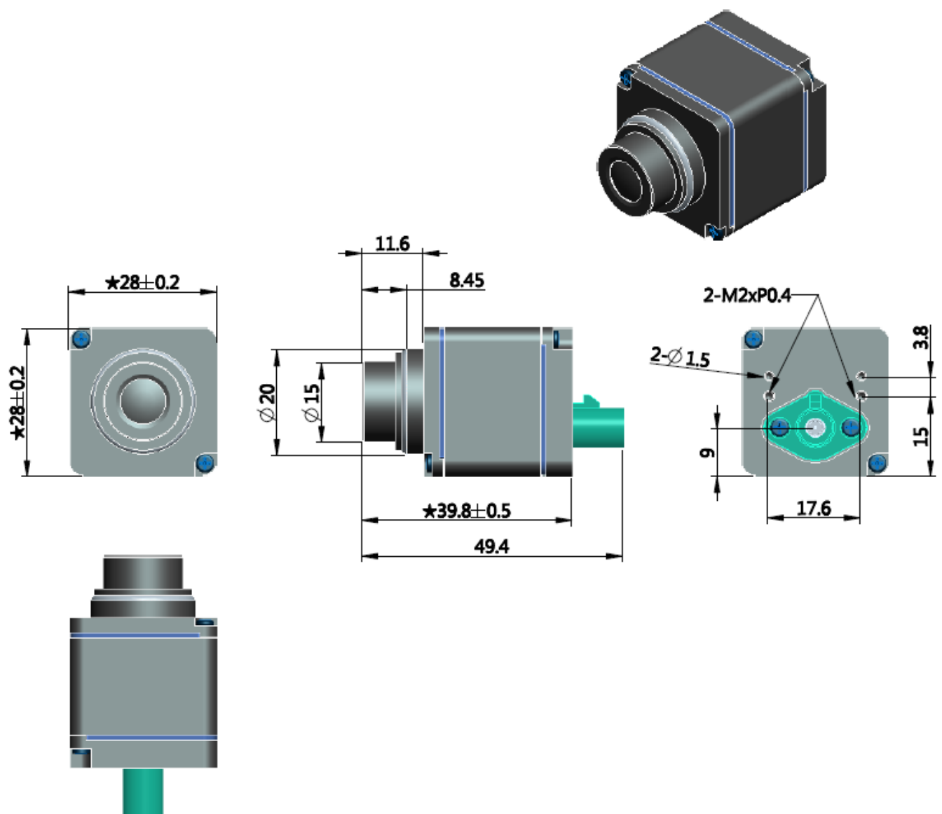
Figure 1. CAM-IMX390-H120-3M GMSL Camera Kit Diagram
