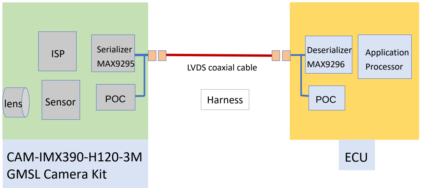
Figure 3. System Configuration
